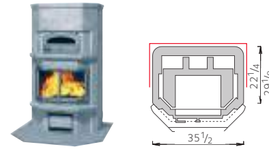
TLU 2137/13 • Weight 4255 lbs • Height 66 1/8"
