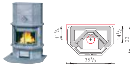
TU1237/51 • Weight 3196 lbs • Height 65"
