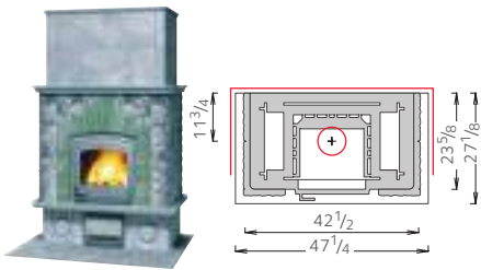
TU2500L • Weight 5247 lbs • Height 76 3/4"
