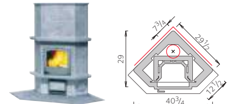
KTU1410/1 • Weight 3042 lbs • Height 65"
