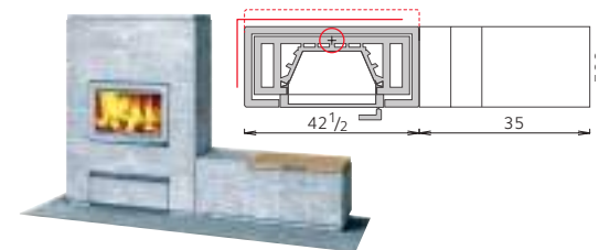
VALKIA + Bench • Weight 3967 lbs • Height 60 1/4" VALKIA T + Bench • Weight 4442 lbs • Depth 23 7/8"
