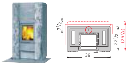
PAHTA/F • Weight 4056 lbs • Height 69 5/8" PAHTA/F T • Weight 4673 lbs • Depth 26 7/8"
