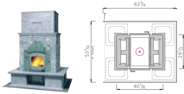
TU2700/2 • Weight 9612 lbs • Height 86 1/2"
