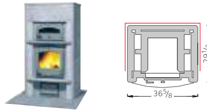
TLU 2000/91 • Weight 4629 lbs • Height 65"
