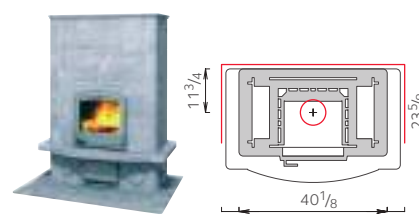
TU2200/4 • Weight 4123 lbs • Height 62 5/8"
