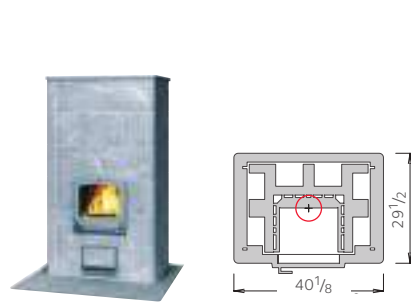
TU2700/4 • Weight 5688 lbs • Height 72"
