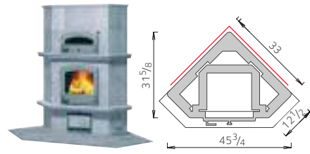
KTLU 2050/1 • Weight 6261 lbs • Height 66 1/8"
