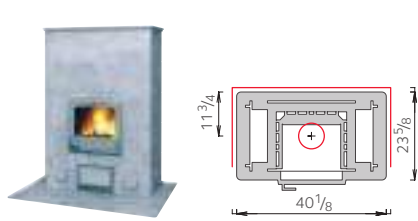
TU2200 • Weight 4056 lbs • Height 60 1/4"
