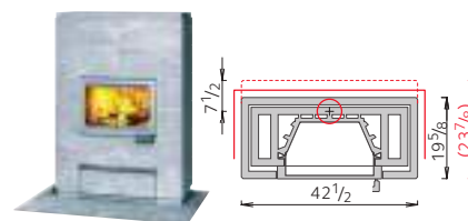
VALKIA • Weight 3350 lbs • Height 60 1/4" VALKIA T • Weight 3825 lbs • Depth 23 7/8"
