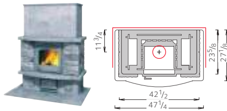
TU2200/1 • Weight 4806 lbs • Height 65"
