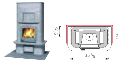
TU1450/1 • Weight 2976 lbs • Height 62 5/8"
